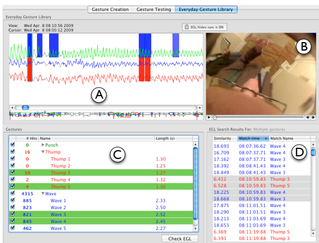
Figure 3. The Everyday Gesture Library tab. A: EGL view with boxes highlighting gesture occurrences; B: EGL video synchronized to EGL view; C: gestures with number of occurrences in EGL (# Hits); D: list of occurrences in EGL for selected gestures.
